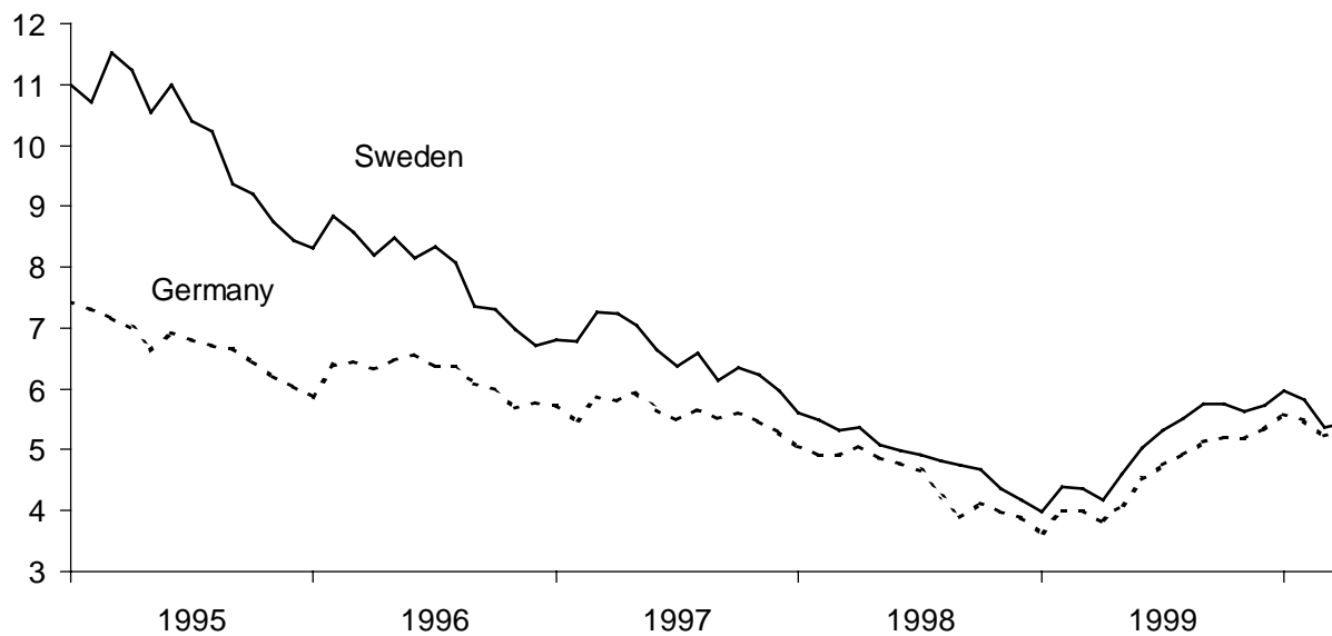
Interest rate on 10 year government bond (from Jan. 1995 to April 2000, monthly)
