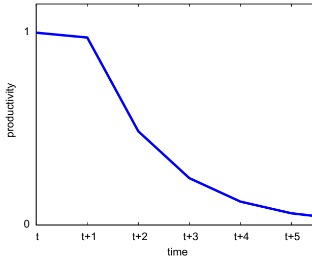
Fig. 1. Remaining stock of capital installed in period t - 1 with quasi-geometric depreciation ( \rho \in (0, 1) ). The parameter values in the example are \rho = 0.05 and \delta = 0.5 .
