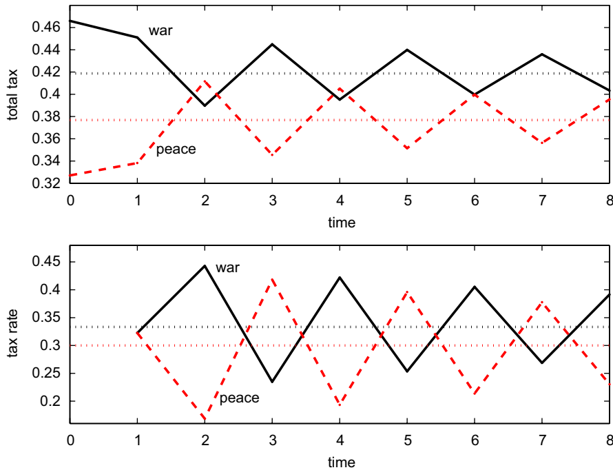
Fig. 3. Upper panel displays the present-value taxes in case of high T_{h,t} (black) and low T_{l,t} (red) spending requirement. The lower panels displays the associated sequence of tax rates. The dotted lines represent steady-state values for taxes conditional on war and peace, respectively. The parameter values underlying this example are \rho = 0.1 , p = 0.5 , and \beta = 0.75 . Moreover, the government expenditures associated with war and peace are chosen so that the Lagrange multipliers become \lambda_h = 2 , and \lambda_l = 1.75 , respectively.
