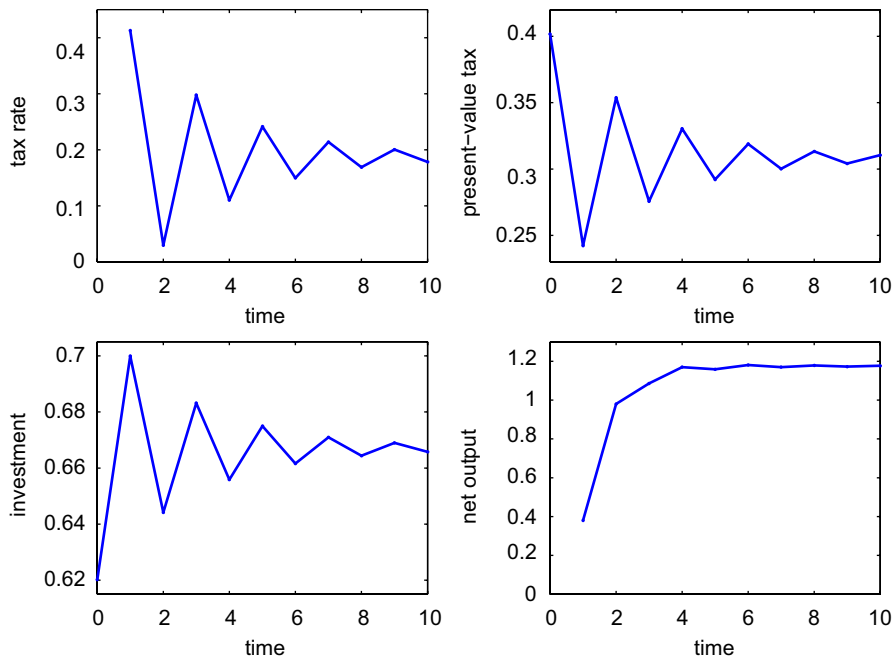
Fig. 2. Ramsey dynamics—an example with accelerating depreciation. The figure displays the dynamic evolution of tax rates ( \tau_t ), present-value taxes ( T_t ), investments ( i_t ), and net output in the optimal Ramsey allocation of Proposition 1. The parameter values underlying the figures are \delta = 0.7 , \rho = 0 , \beta = 0.8 , and an initial stock of installed capital of h_1^0 = 0.25 . Moreover, the government expenditure are such that the Lagrange multiplier is \lambda = 1.3 .
