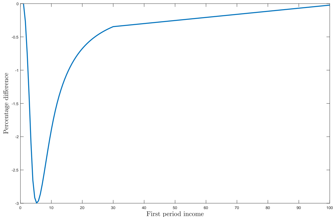
Figure 1: The figure depicts the relative utility loss from not acquiring information in the simple two-period model for \beta = 0.99 and a uniform measure of w \in [1, 10] and R \in [0.9, 1.1]
