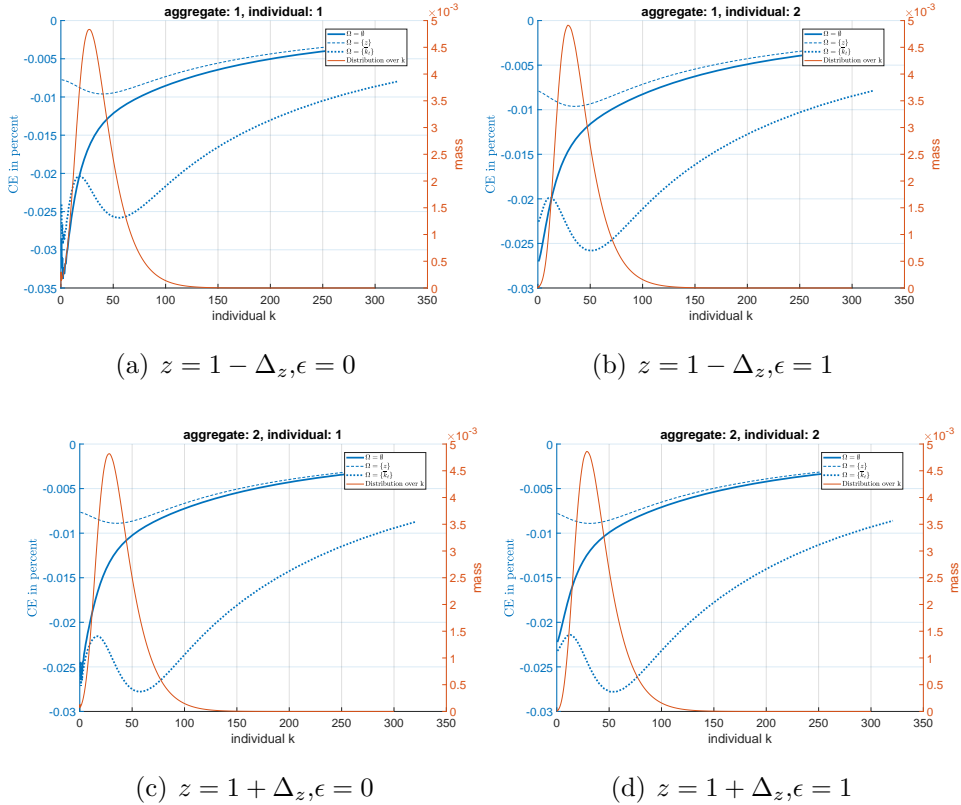
Figure 4: The figure presents CE_{\Omega}(k, \epsilon; \Omega_{max}) , where \Omega_{max} = \{z, k\} is the information set of KS, and \Omega takes three specifications: first, the period-specific cross-sectional mean of k unconditional on z (implying \bar{k} is forecast using an unconditional autoregression for k , solid lines), z only (implying forecasts equal to the mean of k across simulations, conditional on aggregate productivity, dashed lines), and the empty set (implying forecasts of aggregate capital equal its unconditional mean, dotted line). All losses are evaluated at the median of the distribution of aggregate capital conditional on productivity.
